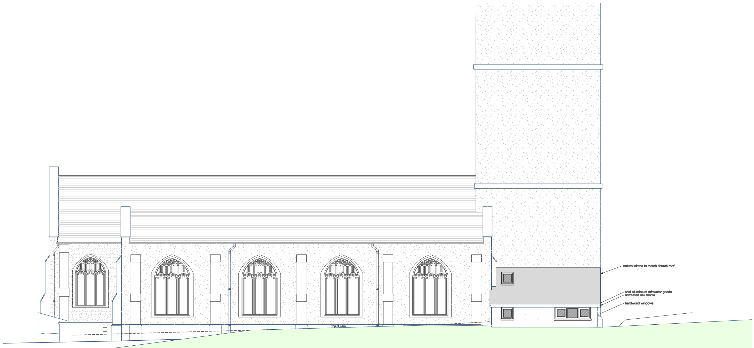
North Elevation
